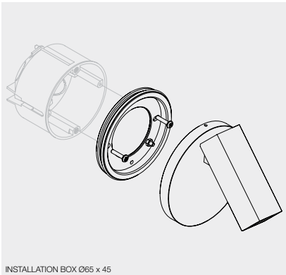
INSTALLATION BOX Ø65 x 45
